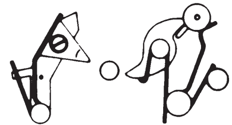
RATCHET SPRING
